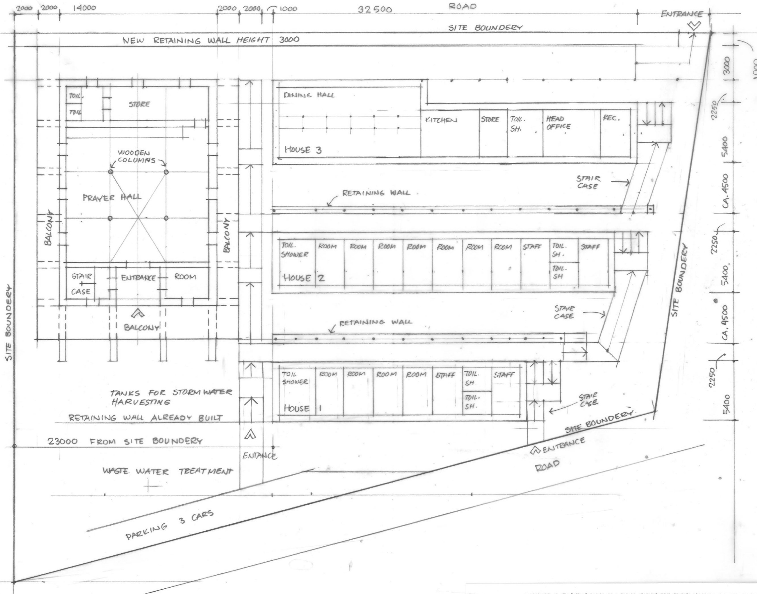
LUMLA BODONG TASHI CHOELING CHARITABLE ORGANIZATION LUMLA, TAWANG, ARUNACHAL PRADESH, INDIA Site layout plan A3 Scale 1:200 Drawing number 1 Anders Nyquist Arkitektkontor AB, Sweden 2014-05-24
